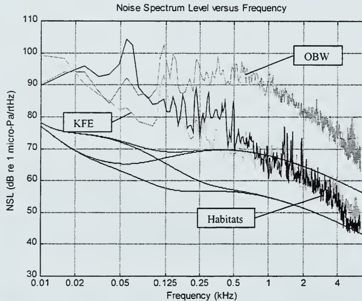
Figure 7.1. Observed 12-Hz-band-average NSL for the OBW, KFE and Habitats exhibits. The estimated NSLs are for w=2 and 10 m/s. Total broadband NLs are: OBW, 124 dB; Habitats, 118 dB; KFE, 112 dB (re 1 \mu\text{Pa} ).
